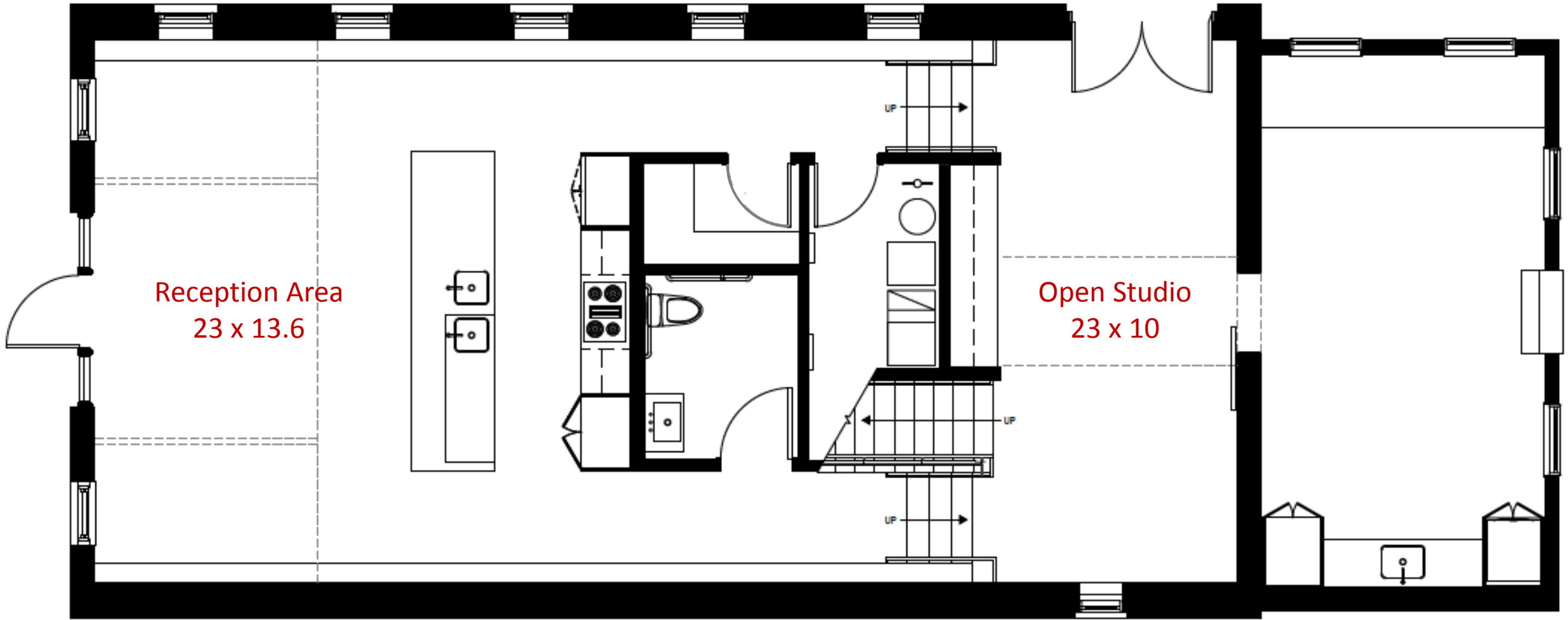
Simons Livery Main Floor
